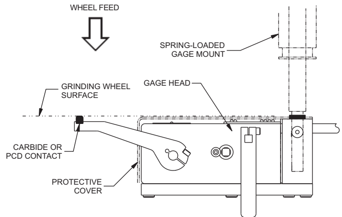
Single wheel position gage on Besley SV6 or V6000 (now made by Giustina) signals the feed endpoint for size control
